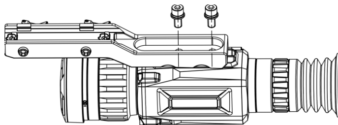
Figure 2-5 Insert Screws
