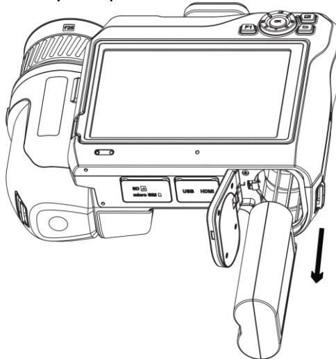
Figure 2-4 Remove Battery
