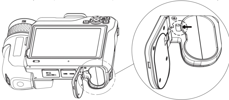
Figure 2-3 Release Battery
