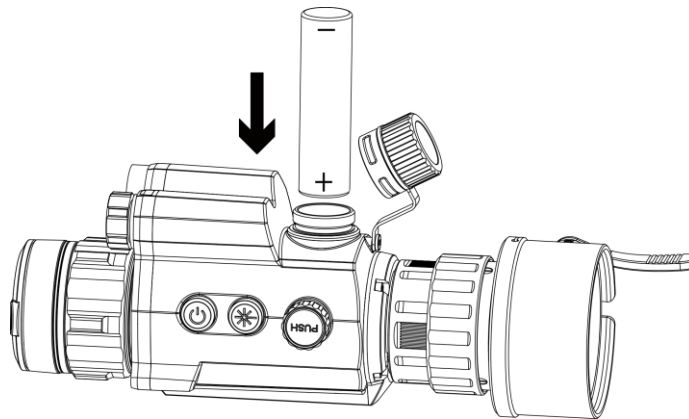
Figure 2-5 Install Battery
