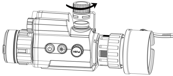
Figure 2-4 Open Battery Cover
