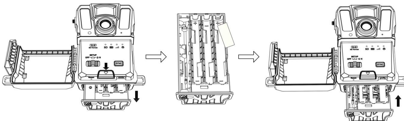
Figure 2-1 Install Batteries
