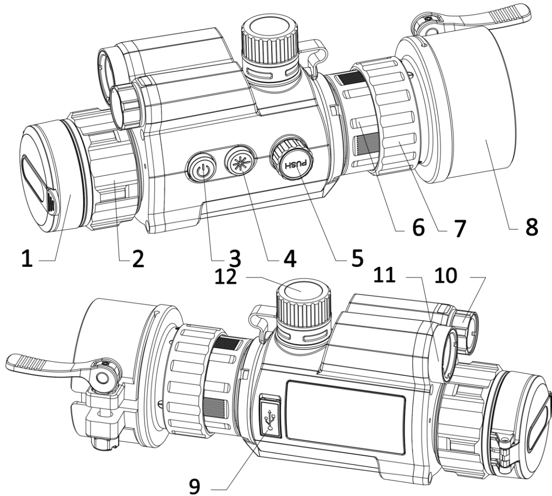
Figure 1-1 Device Appearance
