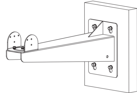
Figure 3-4 Install Bracket
