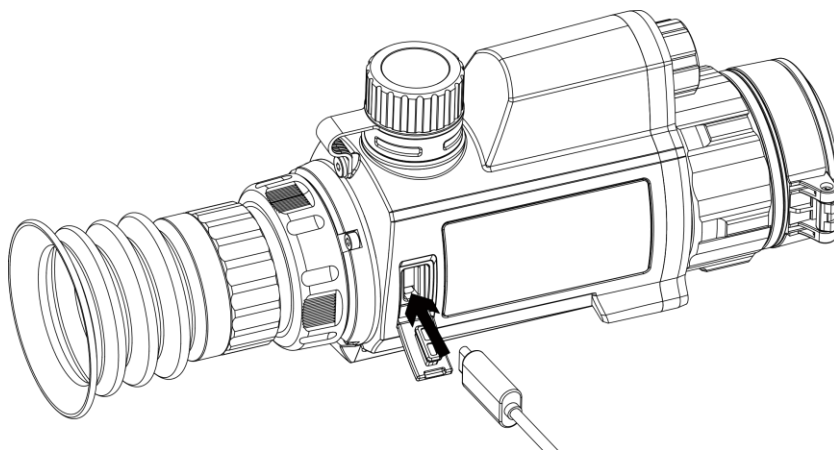
Figur 2-1 Kabeltilkobling
