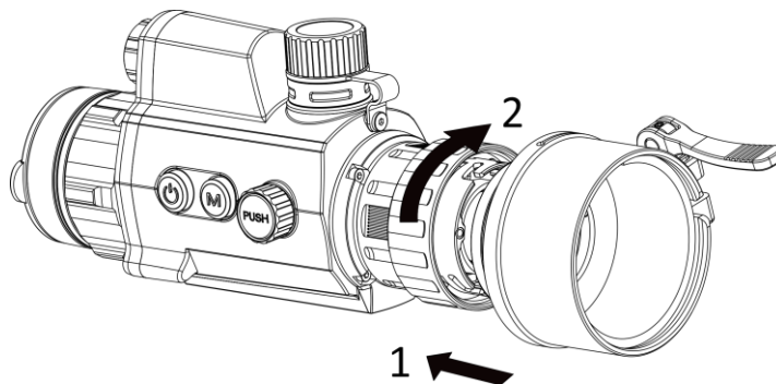
Figure 2-2 Install Adapter
