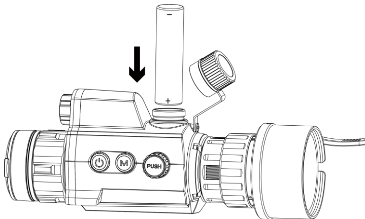
Figure 2-5 Install Battery
