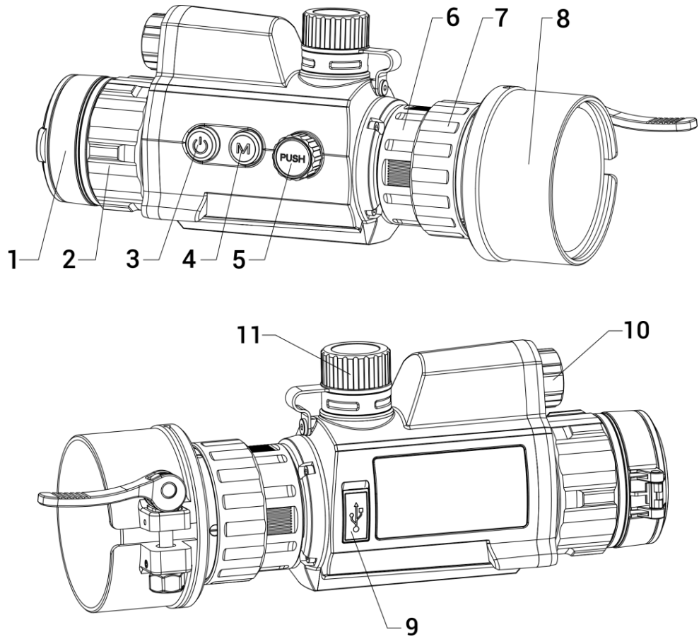
Figure 1-1 Device Appearance
