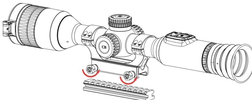
Figur 2-8 Lossa skruvarna
