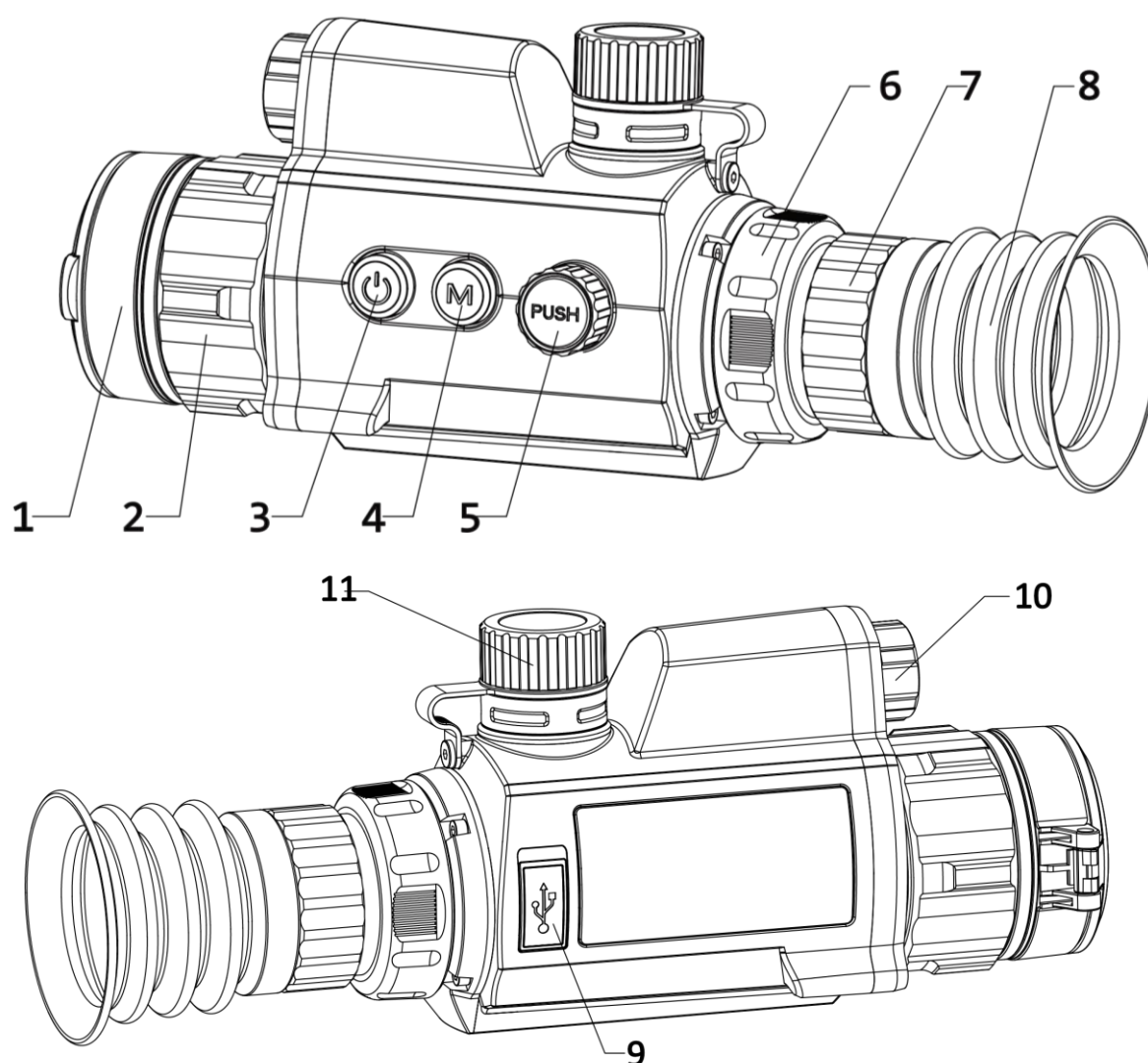
Figure 1-1 Device Appearance
