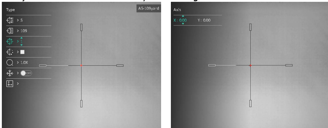
Figure 2-9 Zeroing
