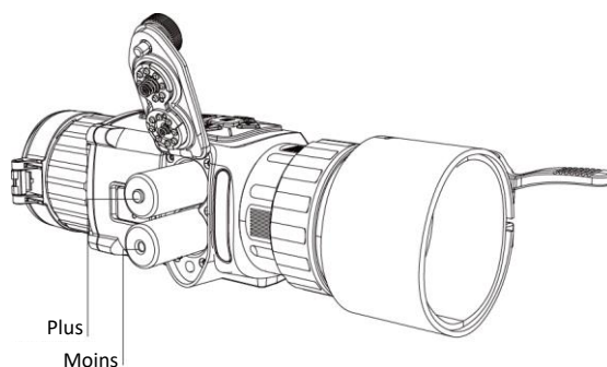
Figure 2-3 Installation des piles
