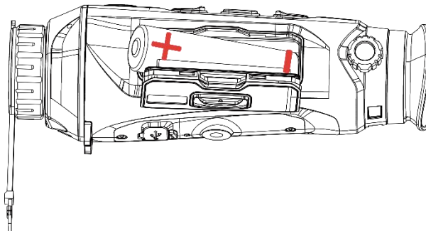
Figure 2-2 Inset the Battery
