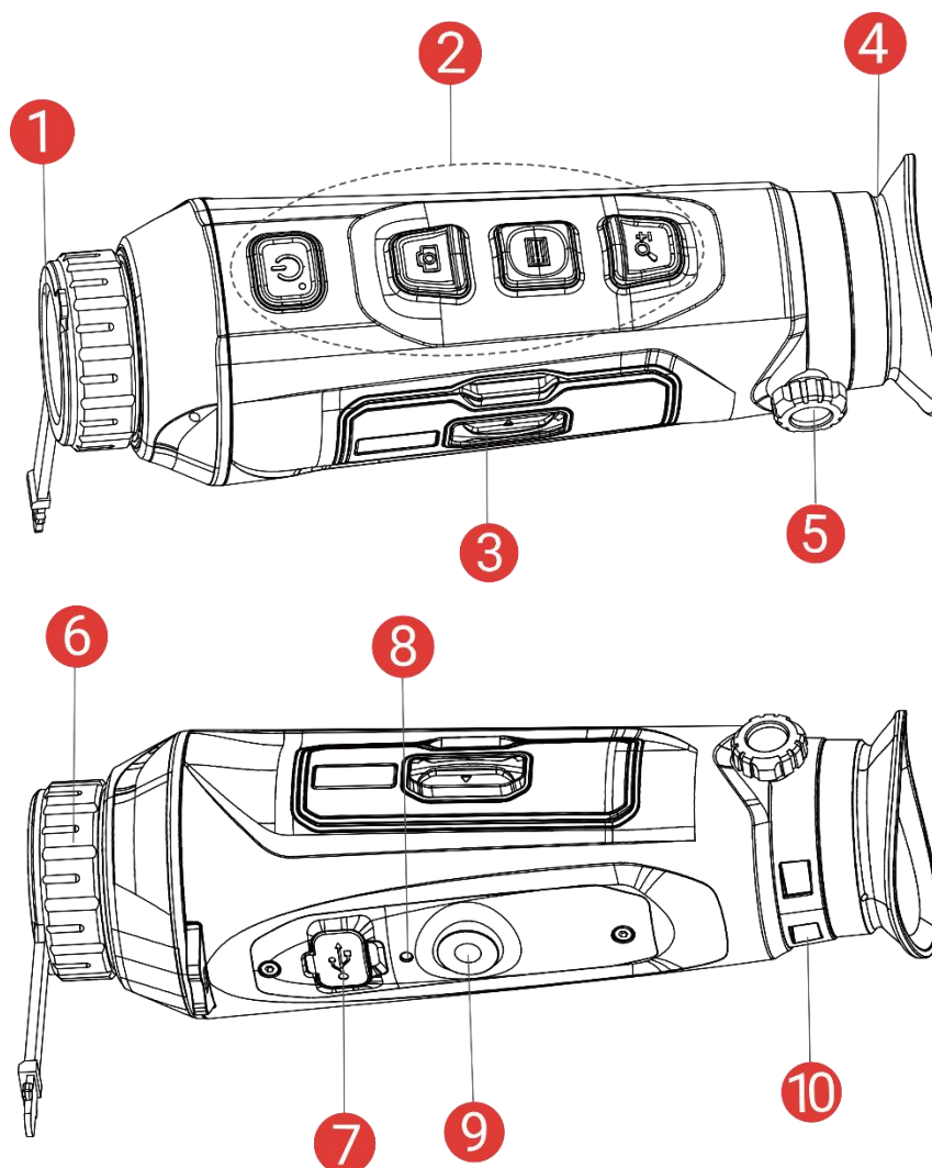
Figure 1-1 Appearance
