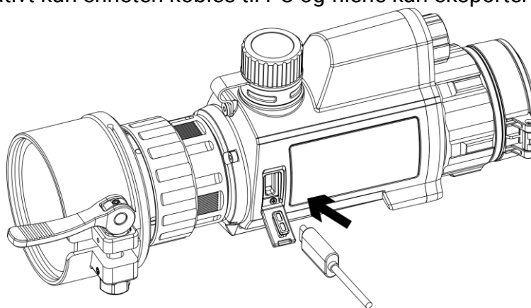
Figur 2-1 Kabeltilkobling
