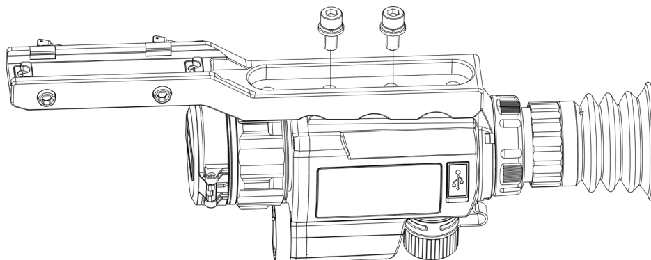
Figure 2-6 Installation des vis
