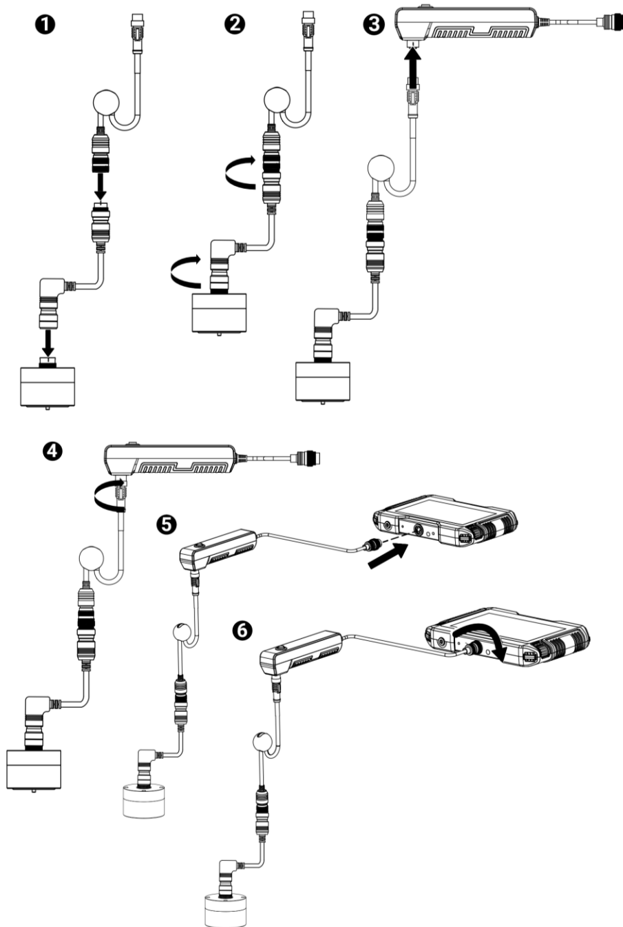
Figure 2-2 Mount the Handheld Sensor
