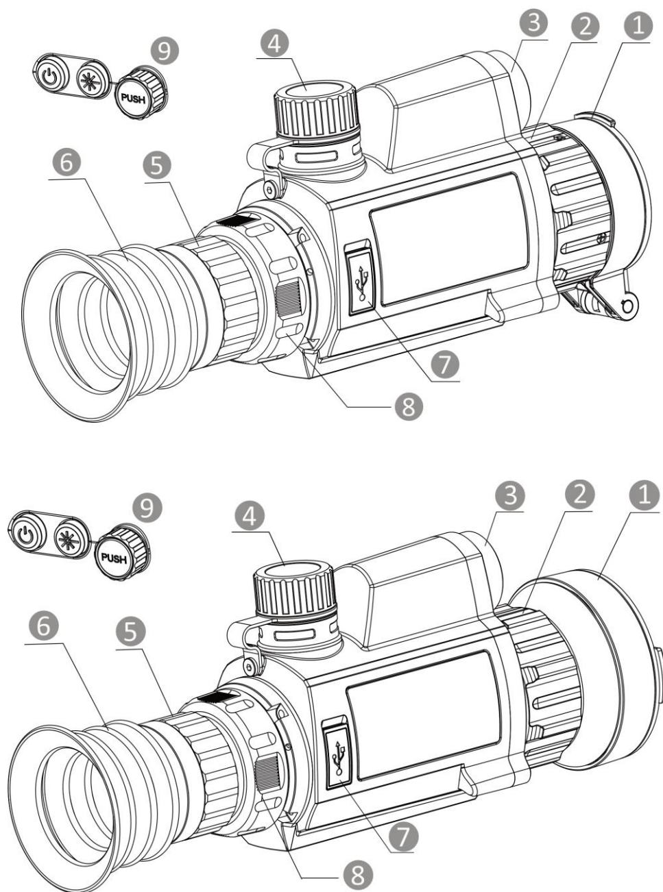
Figure 1-1 Appearance
