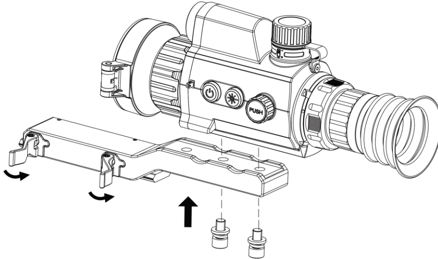
Figure 2-5 Install Screws
