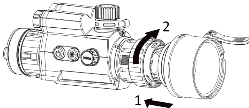
Figur 2-2 Monter adapteren
