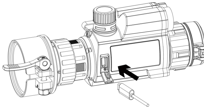
Figur 2-1 Kabeltilkobling
