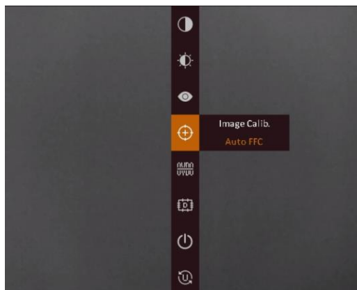
Figure 2-5 Menu Interface
