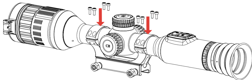
Figure 2-7 Serrage des vis
