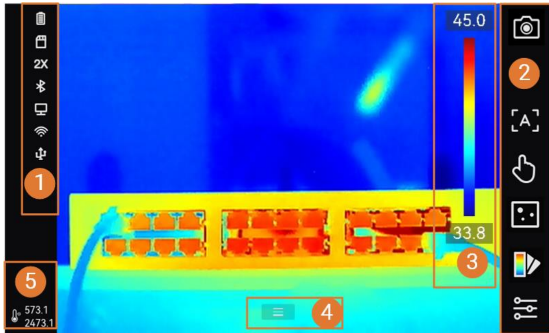
Figure 2-13 Live View
