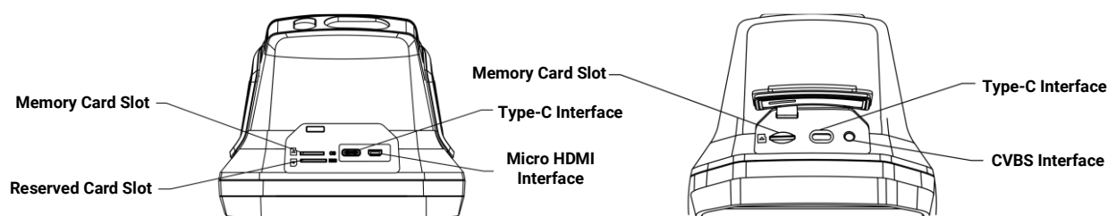
Figure 1-1 Appearance
