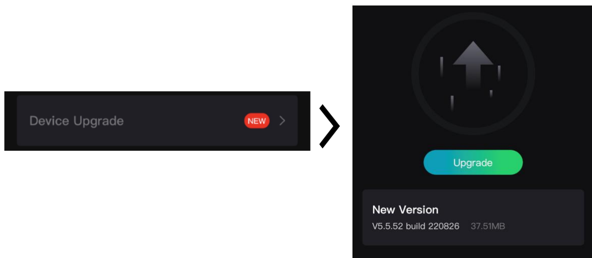
Figur 2-4 Uppgradera firmware
