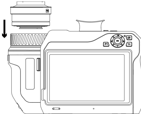
Figure 2-9 Mount Lens
