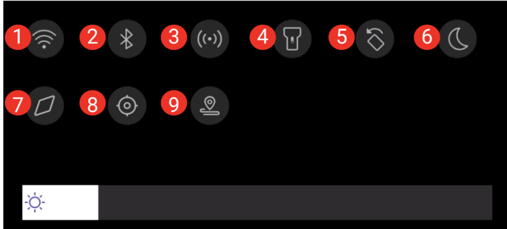
Figure 2-21 Swipe-down Menu
