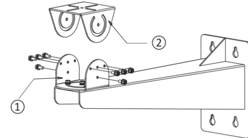
Figure 3-3 Disassemble PT Joint
