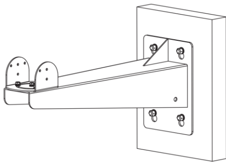
Figure 3-4 Install Bracket
