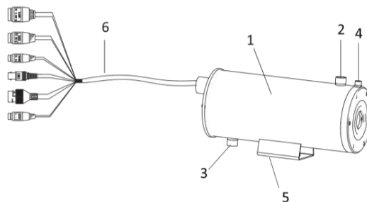
Figure 2-1 Appearance
