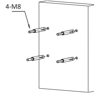
Figure 3-2 Drill M8 Screws into Holes
