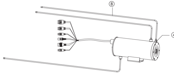
Figure 3-11 Dedusting Installation
