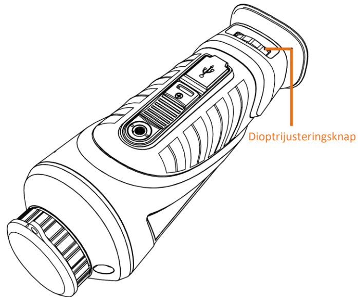
Figur 3-2 Justér dioptri
