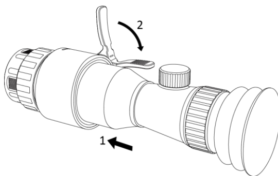
Figura 2-6 Instalar a mira diurna
