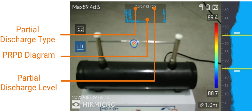
Figure 3-2 Partial Discharge Display
