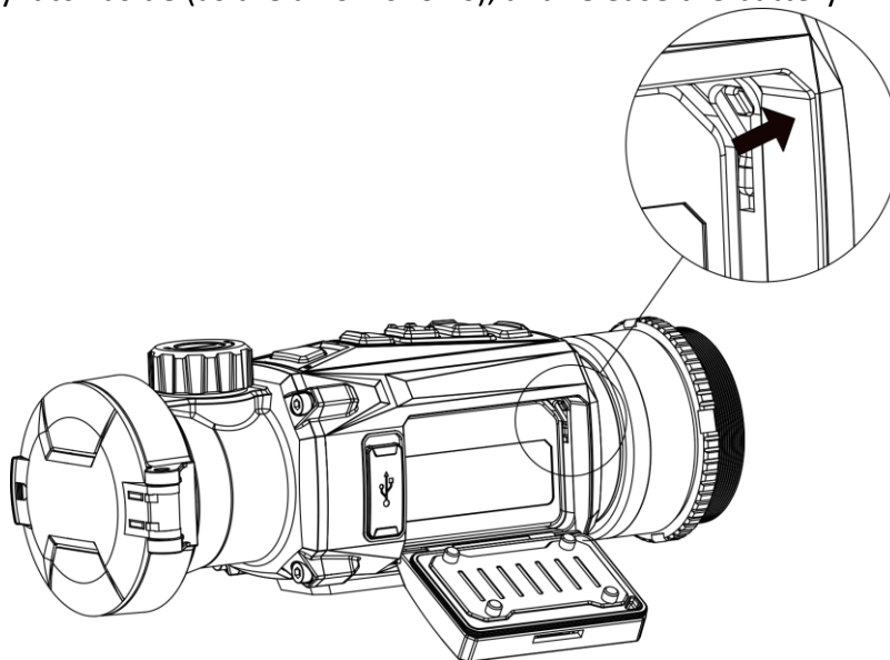
Figure 2-3 Unlatch the Battery Latch
