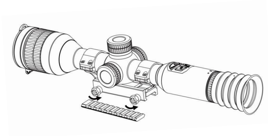
Figur 2-8 Lossa skruvarna
