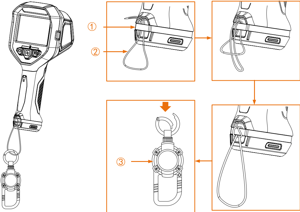
Figure 3-8 Install Lanyards
