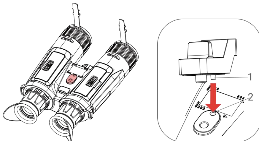
Figure 2-8 Insertion de la colonne
