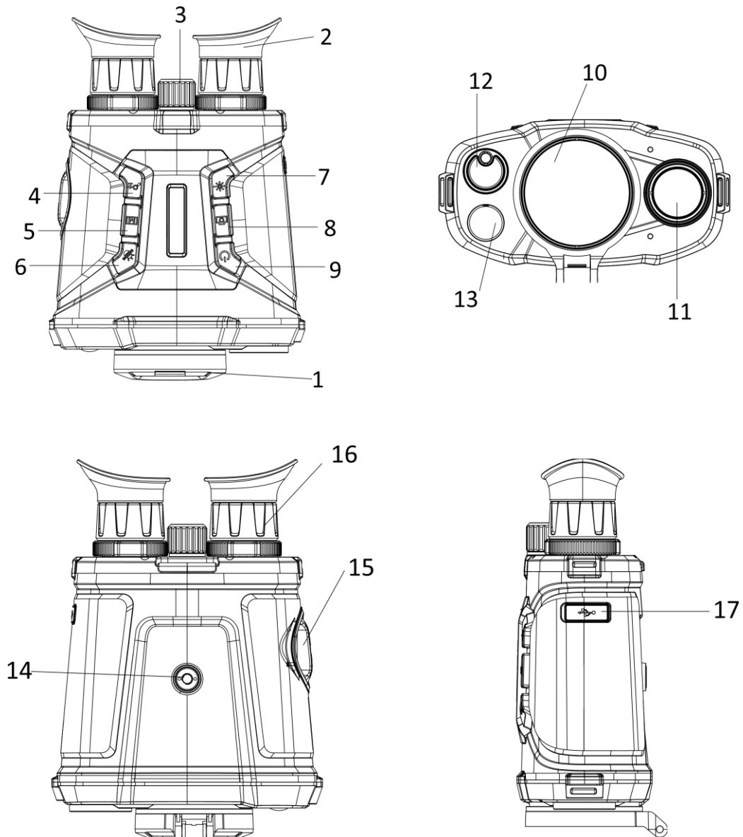
Figure 1-1 Device Appearance
