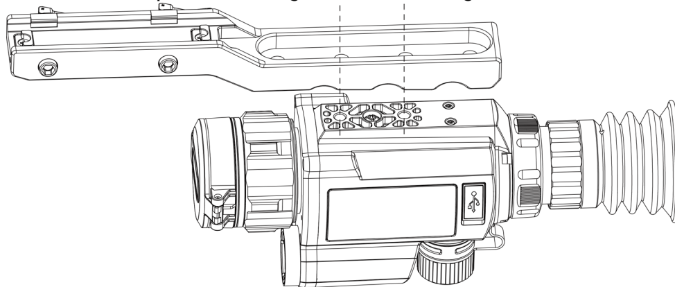
Figur 2-5 Justér installationshullerne
