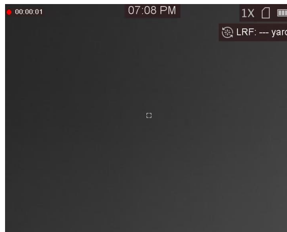
Figure 7-1 Start Recording
