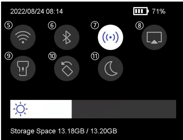
Figura 2-2 Menú desplegable
