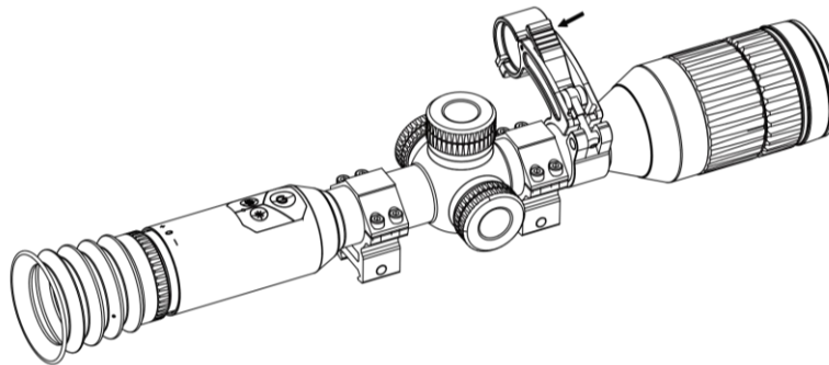
Figure 2-11 Lock the Lever
