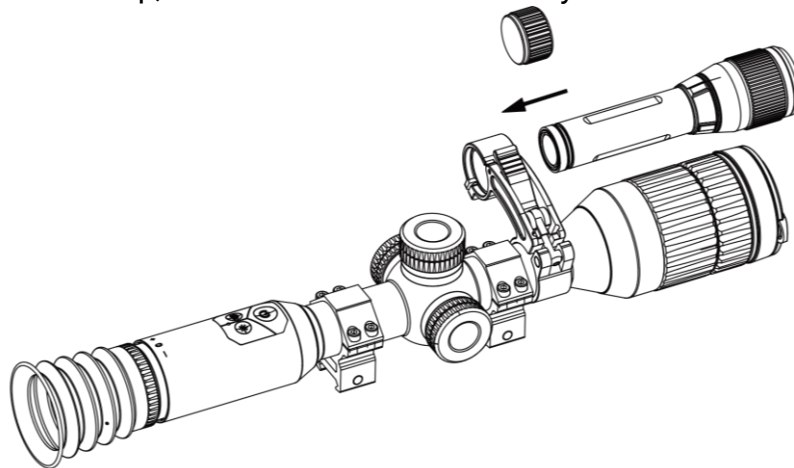
Figure 2-12 Thread the IR Torch
