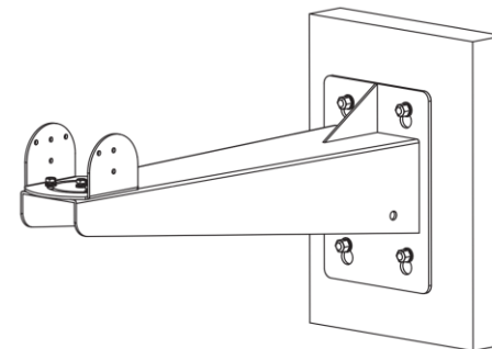
Figure 3-4 Install Bracket
