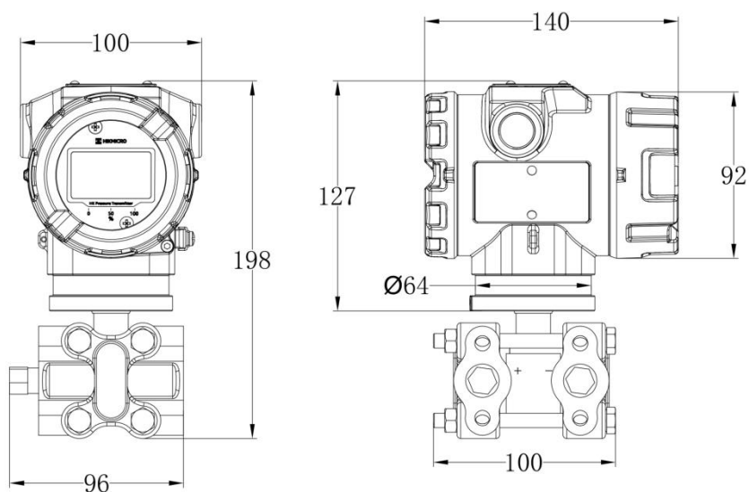
Differential Pressure Transmitter
