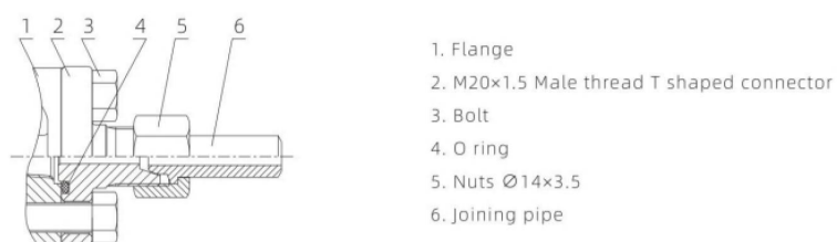
T Shaped Connector with M20x1.5 External Thread
