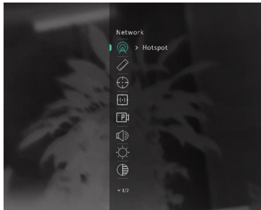
Figure 2-7 Menu principal
