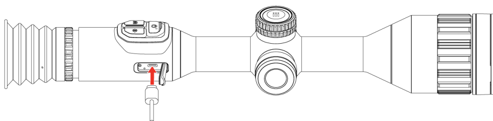
Figur 2-1 Kabeltilkobling
