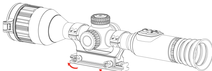
Figur 2-9 Stramme skruene
